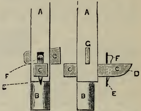
FIG. 133.—Purfling Gauge or Marker (front and side views).
